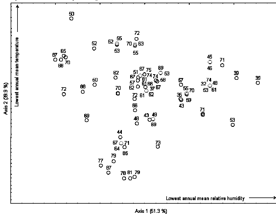
Figure 2 Scatter plots of the first two multifactorial axes for six climatic variables representing the climate of origin for the 72 RH_{50} considered. Percentages in each axis refer to the amount of variation accounted for by the first and second axes in the multifactorial analysis.
